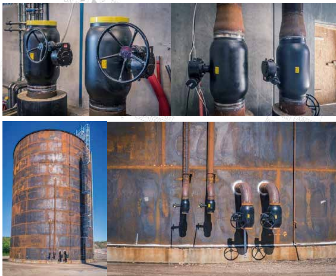
Hobro District Heating Station: BROEN Ballomax® valves DN250-400 – Designed to last.
